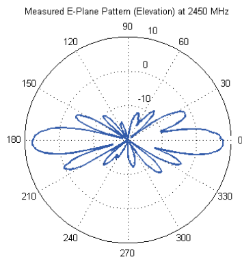
E-Plane Radiation Pattern
