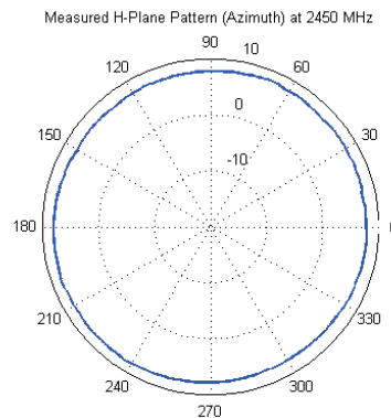
H-Plane Radiation Pattern
