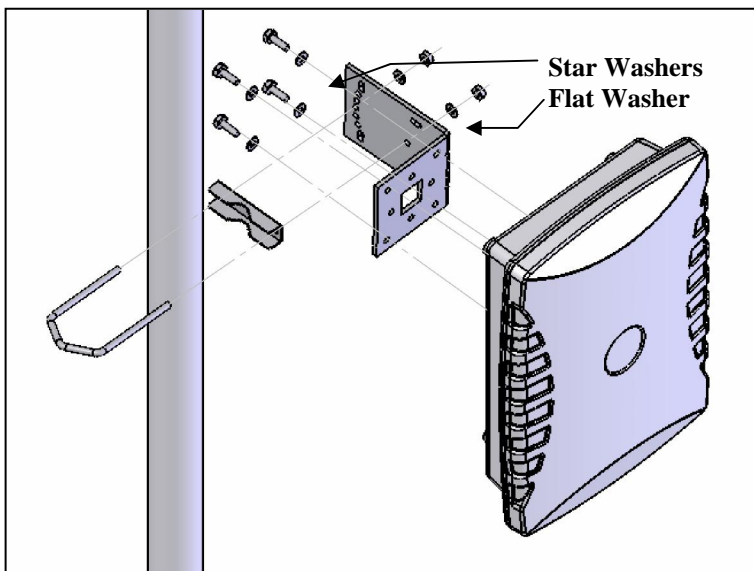
Figure 8. Mast mounting
